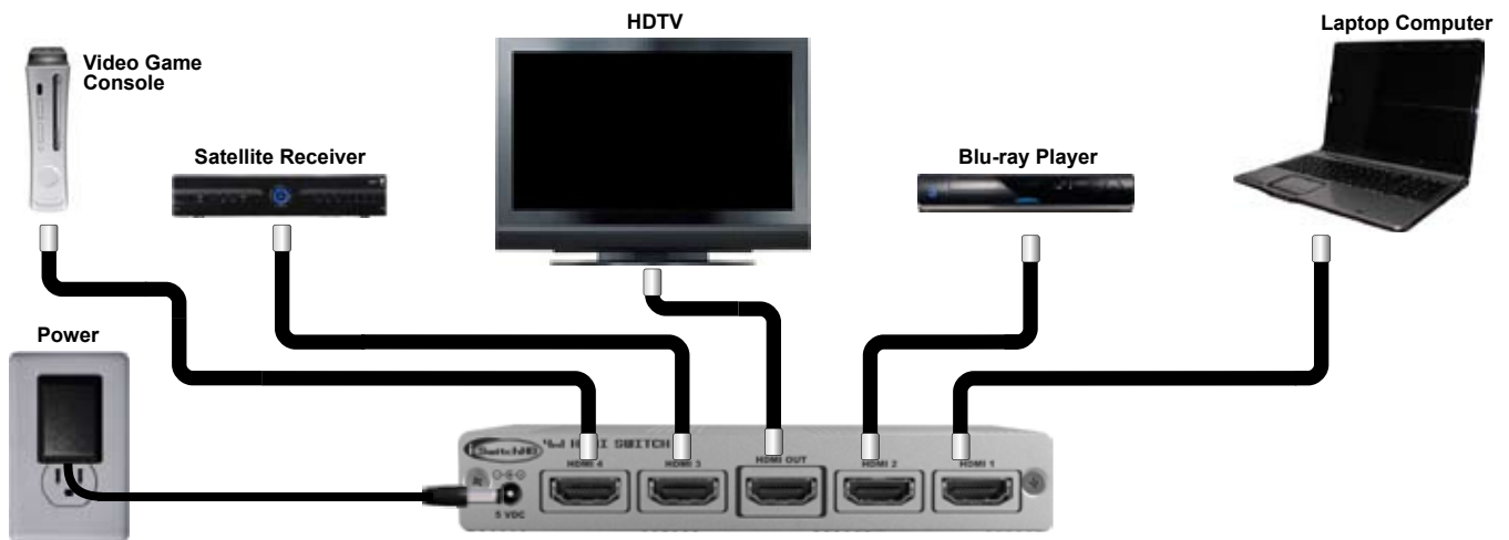
Figure 1 - Connecting the iSwitchHD-CE to power, a display, and various sources such as a Satellite Receiver, Blu-ray, video game console, and computer.
